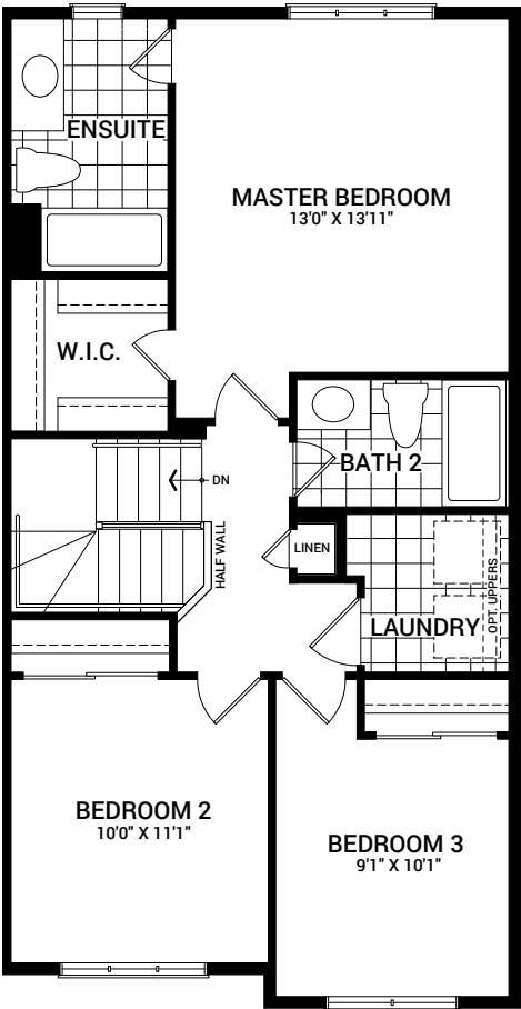
SECOND FLOOR PLAN B
